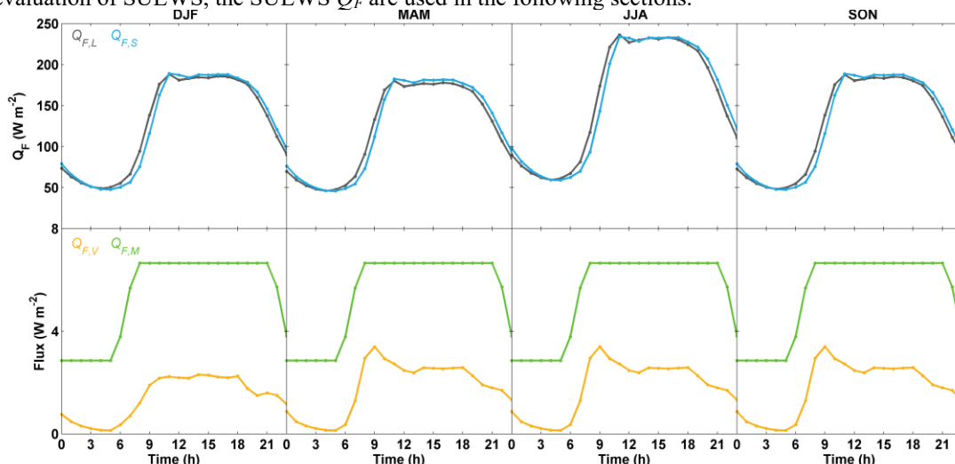
Figure 4: Seasonal mean diurnal variations of Q_F at XJH estimated by LQF and SUEWS (section 2.2), LQF metabolic heat ( Q_{FM} ) and vehicle heat ( Q_{FV} ) emissions.
