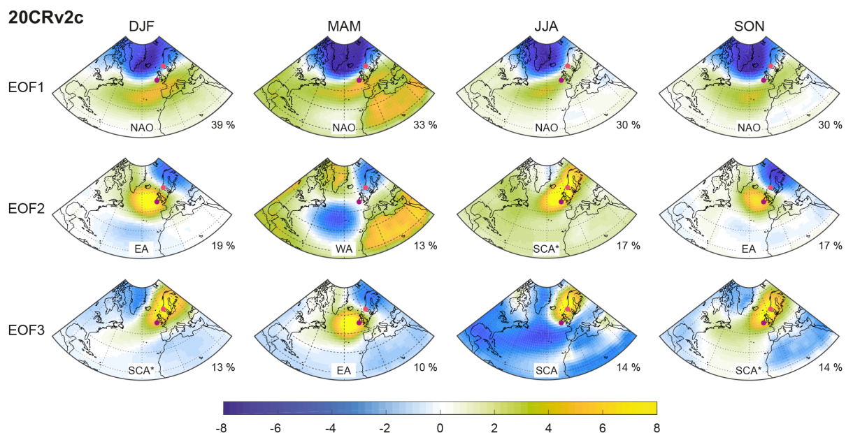
Figure 1. EOF loadings based on monthly SLP data (20CRv2c dataset; Compo et al., 2011). Each column represents a 3-month season. The percentages at the bottom right of each map are the variability explained by the corresponding EOF (rows) at any given season (columns) as shown in Table S2. The text at the bottom of each map identifies the observed pattern. Pink (purple) dots show the location of Bergen Florida (Valentia Observatory) stations as listed in Table 1. Figures S1–S4 show the same maps for the other four reanalysis products in Table 2.
