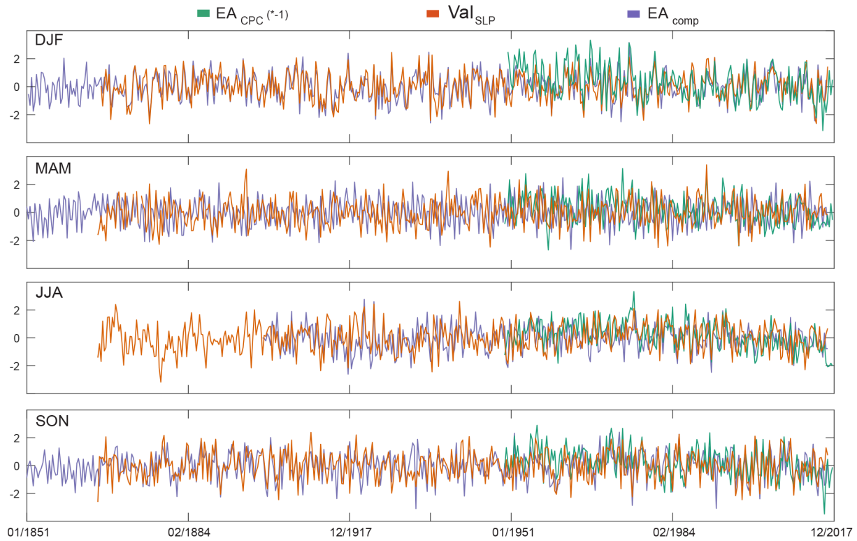
Figure 3. Monthly series of EA_{comp} , the instrumental data ( Val_{SLP} ) and the EA from the CPC ( EA_{CPC} ; CPC, 2012) for each 3-month season. Note that the CPC series have been inverted for an easy visual comparison.
