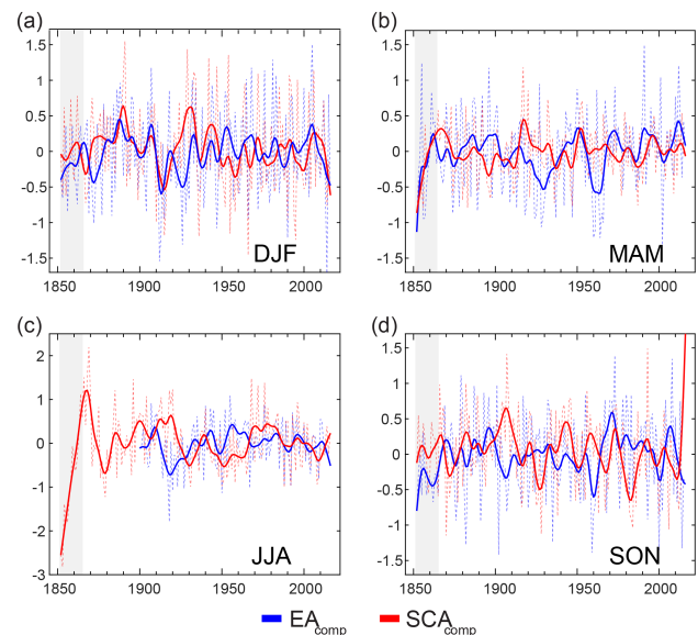
Figure 6. Seasonally averaged EA_{comp} (dashed blue line) and SCA_{comp} (dashed red line) and decadal EA_{comp} (blue solid line) and SCA_{comp} (red solid line). (a) Winter (DJF); (b) spring (MAM); (c) summer (JJA); (d) autumn (SON). A 10-year bandpass filter has been used to obtain the decadal series. Note that in (b) the red lines correspond to WA_{comp} instead of SCA_{comp} . Note the different y scale for summer indices. The grey band indicates the period of low confidence of our composite series (see Methods section for details).
