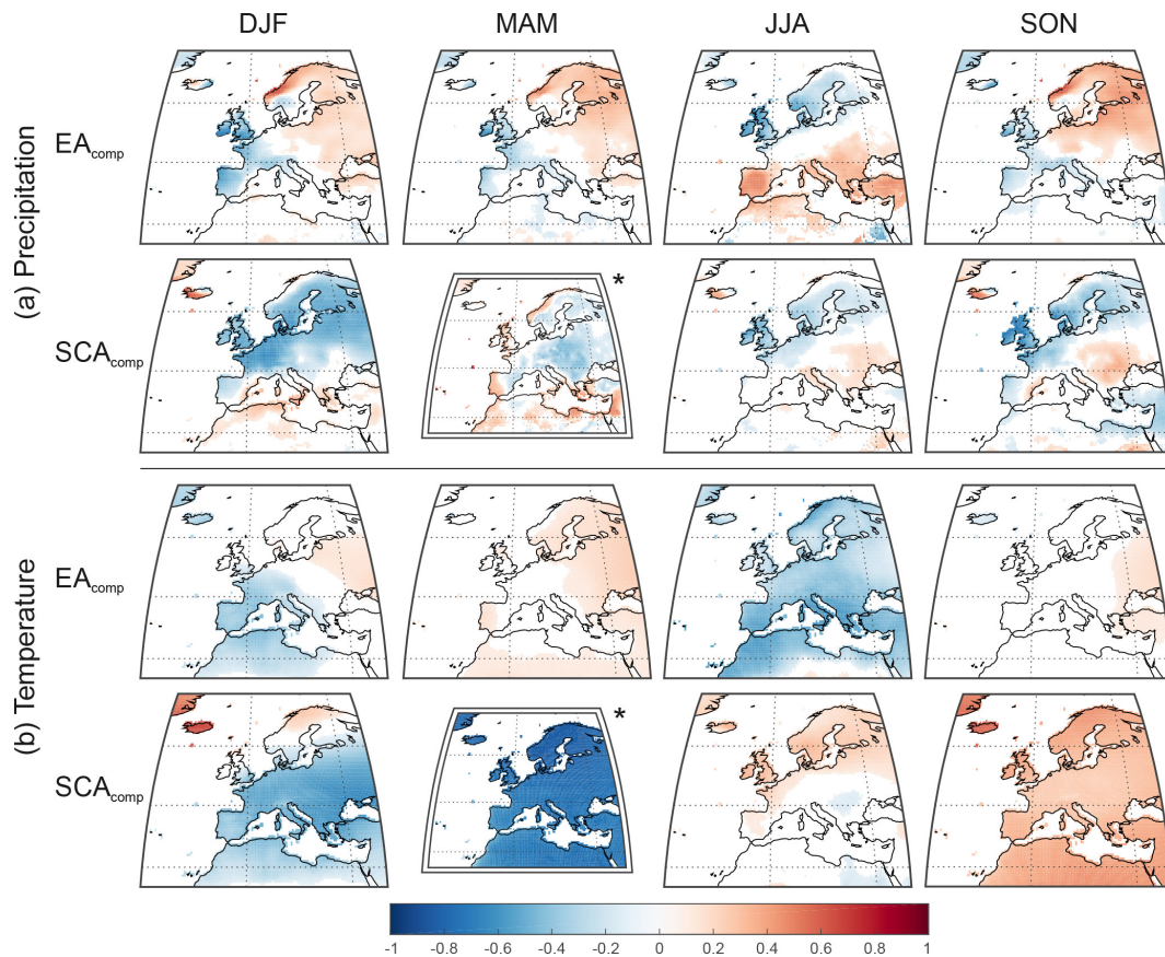
Figure 8. Correlation distribution maps between the monthly precipitation (a) and surface air temperature (b) and our monthly composites ( EA_{comp} and SCA_{comp} ) between 1902 and 2016. Climate data from the CRU-TS4.01 global climate data set (Harris et al., 2014). Positive correlations are shown in red and negative correlations are shown in blue (see colour bar). Correlation coefficients are Spearman rank coefficients. SCA_{comp} MAM maps (marked with an asterisk) correspond to the WA pattern.
