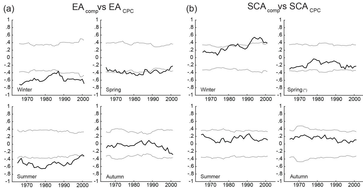
Figure 7. Running correlations as in Fig. 5 between our composite series and the CPC indices. (a) EA_{comp} and EA_{CPC} ; (b) SCA_{comp} and SCA_{CPC} . The window size is 30 years and is defined from i to i + 30 , where i is the oldest month. Dashed lines indicate the 0.01 significance thresholds.
