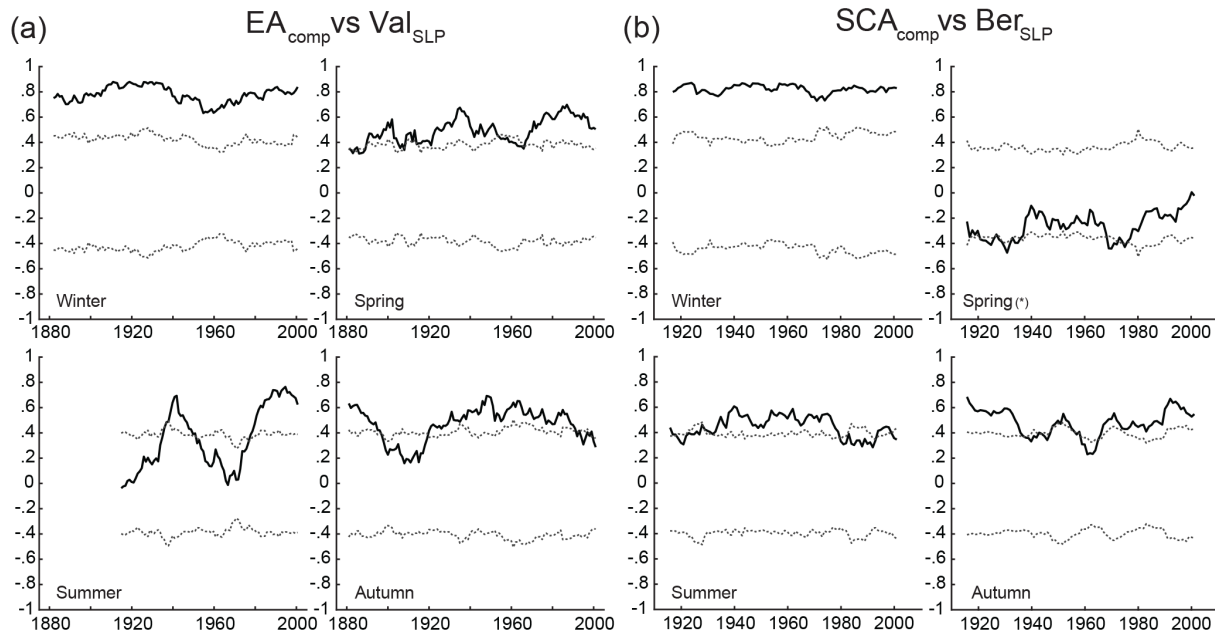
Figure 5. Running correlations between our composite series and the instrumental records. (a) EA_{comp} and Val_{SLP} ; (b) SCA_{comp} and Ber_{SLP} . The window size is 30 years and is defined from i to i + 30 , where i is the oldest month. Dashed lines indicate the 0.01 significance thresholds. Note that spring in panel (b) corresponds to the WA index instead of the SCA.
