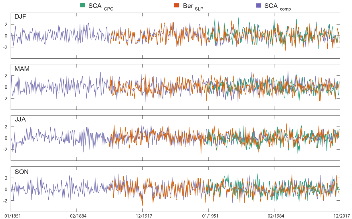
Figure 4. Same as in Fig. 3 for SCA_{comp} , instrumental data ( Ber_{SLP} ) and the SCA from the CPC ( SCA_{CPC} ; CPC, 2012).
