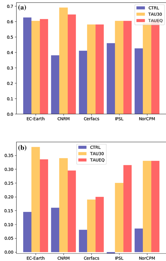
Fig. 14 Bjerknnes feedback components for each model, coloured according to experiment: CTRL (blue), TAU30 (yellow) and TAUEQ (red). Bars show a effect of western wind stress on eastern mixed layer depth with a 1 month lag and b effect of eastern mixed layer depth on local SST
