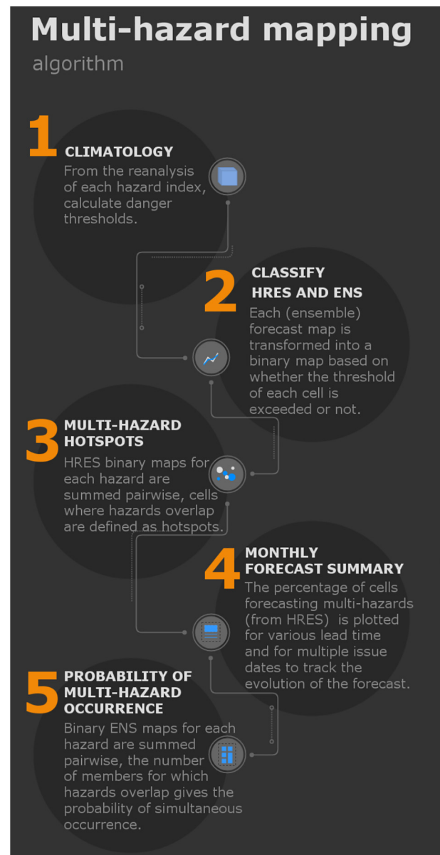
Fig. 1. Workflow illustrating the algorithm for multi-hazard mapping. Image made using https://www.draw.io/ .
