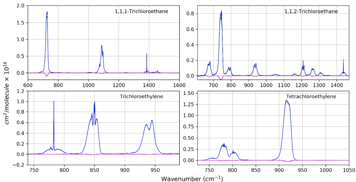
7 8 Figure 12. Absorption from NIST [17] in blue and PNNL [13] in green. The residual (magenta) 9 between PNNL and NIST is given in the same scale.
