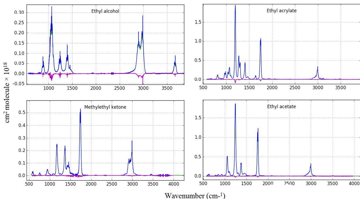
7 Figure 3. Comparison of PNNL [13] (green) and NIST [17] (blue) spectra. Residuals (PNNL-NIST) are 8 displayed on the same scale in magenta. Intensity differences are apparent in the stronger bands.
