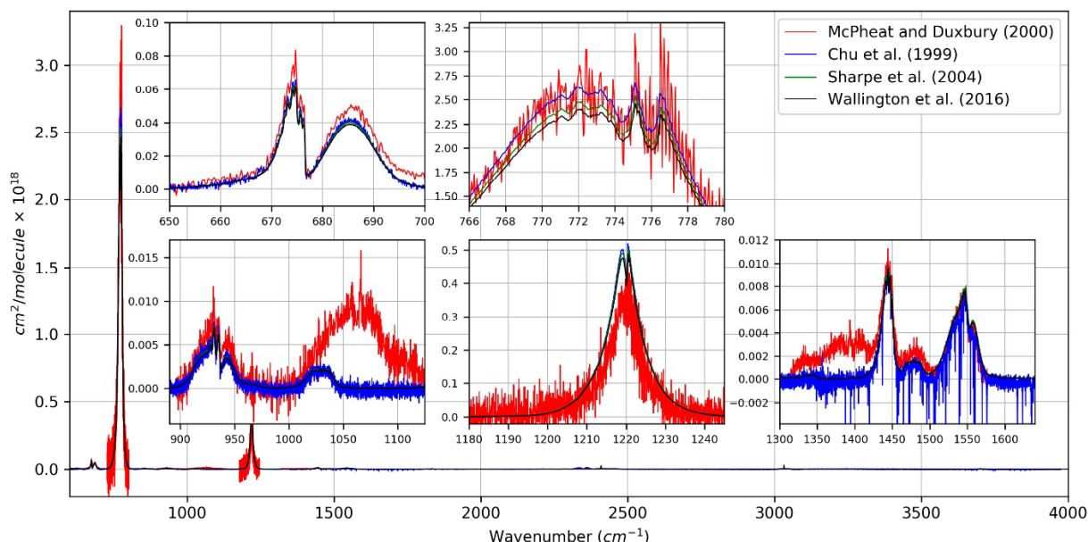
14 15 Figure 14. Absorption cross-section comparison for chloroform. The insets show the difference 16 in the band shapes at 1000 \text{cm}^{-1} and 1500 \text{cm}^{-1} . The contaminant lines at 1400-1600 \text{cm}^{-1} are due 17 to water vapor absorption.
