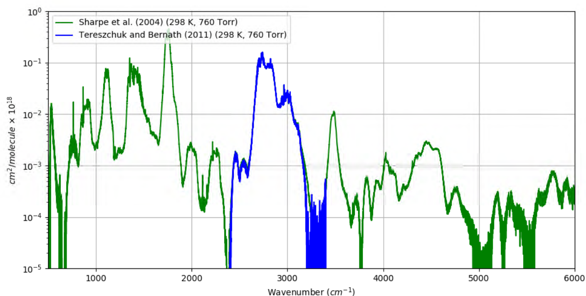
2 Figure 2. Comparison of the spectral coverage for the acetaldehyde (acetylaldehyde) data from PNNL 3 [13] which are new to HITRAN and those from Tereszchuk and Bernath [82] represented in the 4 HITRAN2012 [6] database. The HITRAN2016 set is a combination of the spectra from these two 5 sources.
