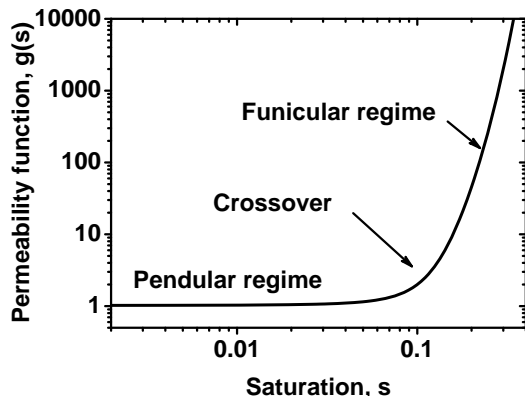
Figure 13. Permeability function g(s) versus saturation s at \alpha_g = 16.5 , \beta_g = 1.65 and f_0 = 1 .
