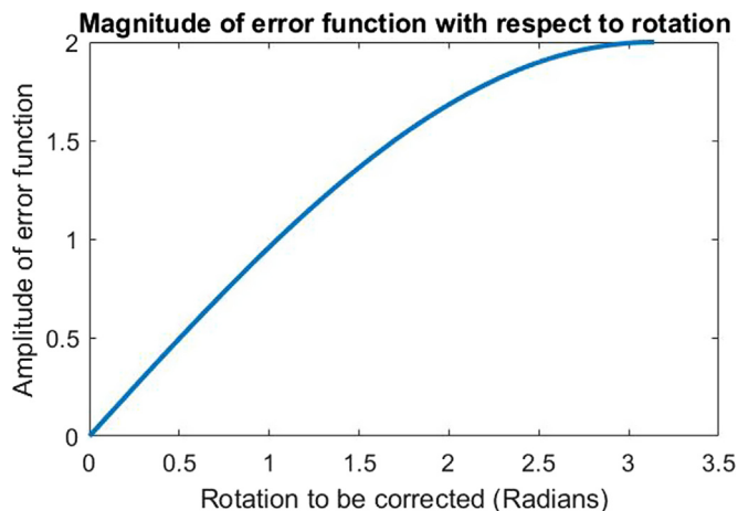
Fig. 1. Algorithm Convergence.
