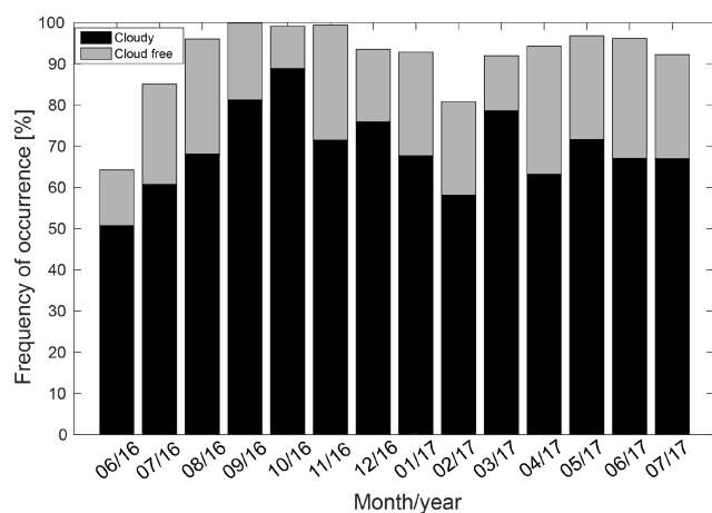
Figure 4. Cloudnet data availability for Ny-Ålesund for June 2016 to July 2017. Grey bars correspond to clear-sky profiles, black bars to cloudy profiles, and white space means no Cloudnet data availability.
