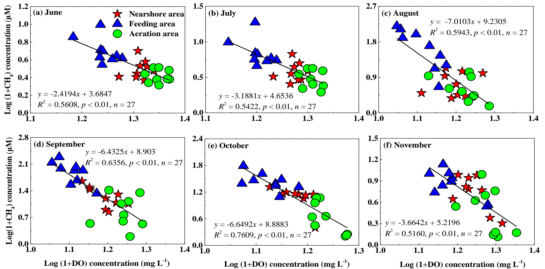
Figure 6. Relationship between the CH 4 concentrations and dissolved oxygen (DO) concentration in the surface water (20 cm depth) at shrimp ponds in the Min River estuary during each sampling campaign. Parameter bounds on the regression coefficients are 95% confidence limits.
