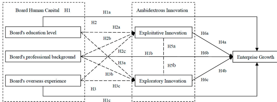
Figure 1. Theoretical Model.
