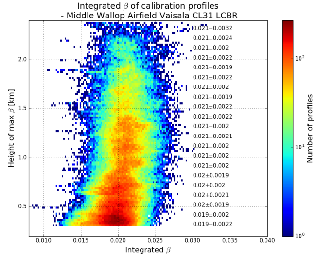
Figure 6. 2-D histogram of integrated attenuated backscatter with range, with height-dependent multiple-scattering correction applied. Darker colours (towards red) indicate a higher density of profiles. The values shown along the right-hand side give the mean \pm SD of the integrated attenuated backscatter (units \text{sr}^{-1} ) at 100 m intervals.
