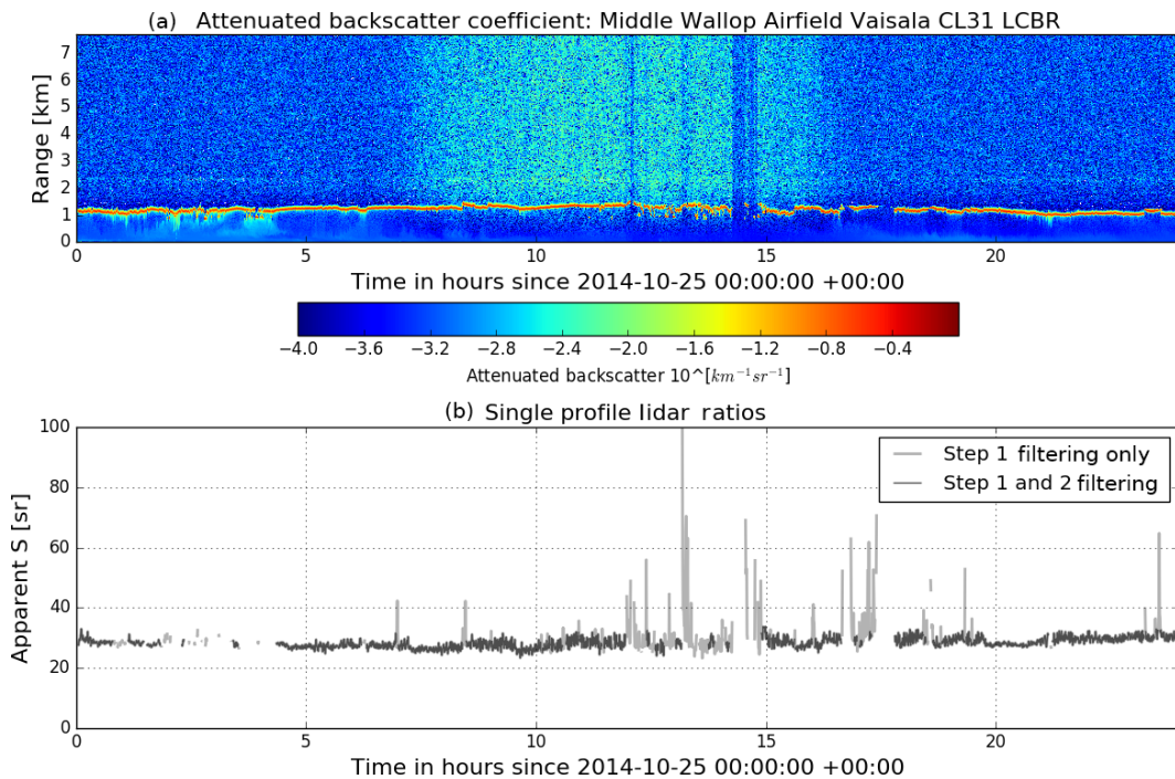
Figure 3. (a) Uncalibrated attenuated backscatter vertical profiles (colours shown on a log scale) for 25 October 2014 from a CL31 ceilometer at Middle Wallop airfield ( 51.1489^{\circ} N, 1.5700^{\circ} W) and (b) the apparent lidar ratio for the same day. In (b), the grey line shows the apparent S for profiles that pass the step 1 filtering of the calibration algorithm and the black line shows the profiles that pass the step 2 filtering and are used to calculate the calibration coefficient.
