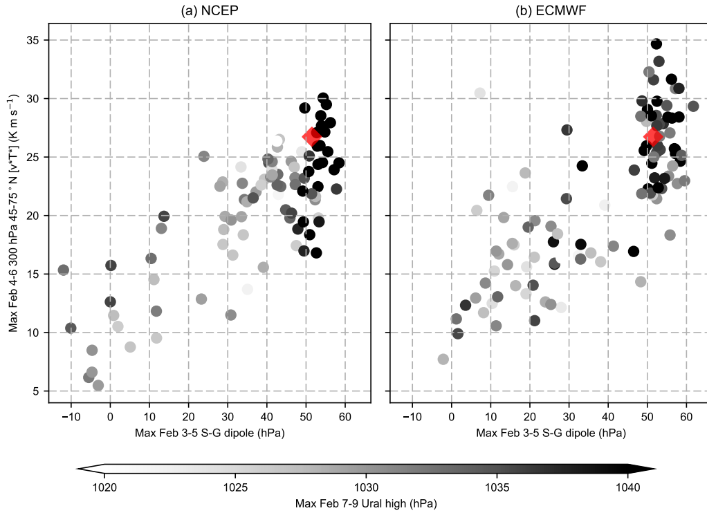
544 Figure 7. Scatter plots of maximum 4–6 February 300 hPa [v^*T^*] versus maximum 3–5 545 February mean S-G dipole for (a) NCEP ensembles from 29 January to 3 February ( n = 96 ), and 546 (b) ECMWF ensembles from 29 January and 1 February ( n = 102 ). The points are coloured by 547 the corresponding maximum 7–9 February Ural high strength. The verifying ERA-Interim value 548 is shown with a red diamond.
