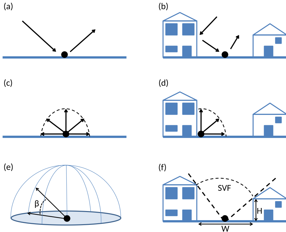
Fig. 1. Radiation components in an open field and street canyon and, SVF calculations illustrated. (a) Short wave radiation in an open field. (b) Short wave radiation in a street canyon. (c) Emission of long wave radiation in an open field. (d) Emission of long wave radiation in a street canyon. (e) SVF calculated in 3D; where, \beta is the angle from the center point to the maximum obstacle height (Eq. (2)). (f) SVF in a 2D street canyon; where W is the street width and H is the building height (Eq. (1)). Figures are adapted from (De Wolff, 2008; Hämmerle et al., 2011).
