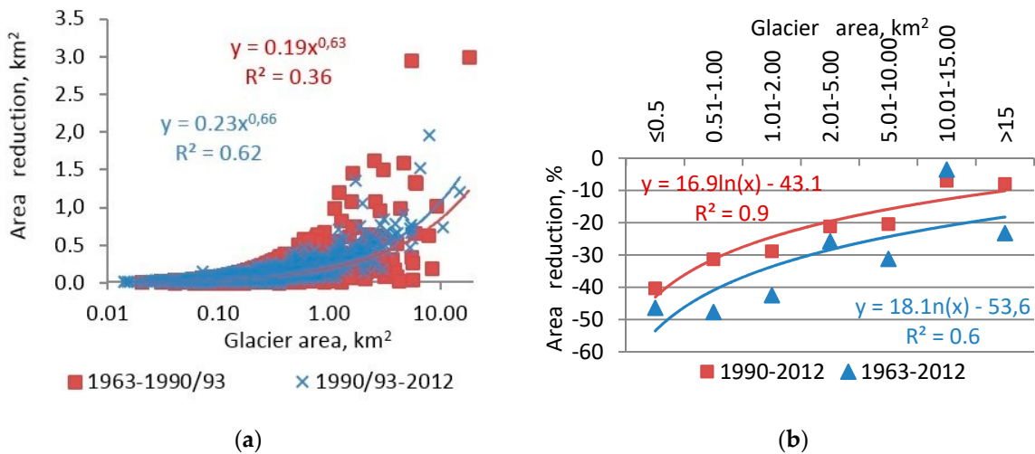
Figure 5. Scatter plot of (a) absolute glacier area loss and (b) relative area loss over the two assessment periods versus the initial glacier areas as in 1962/63 and 1990/93.
