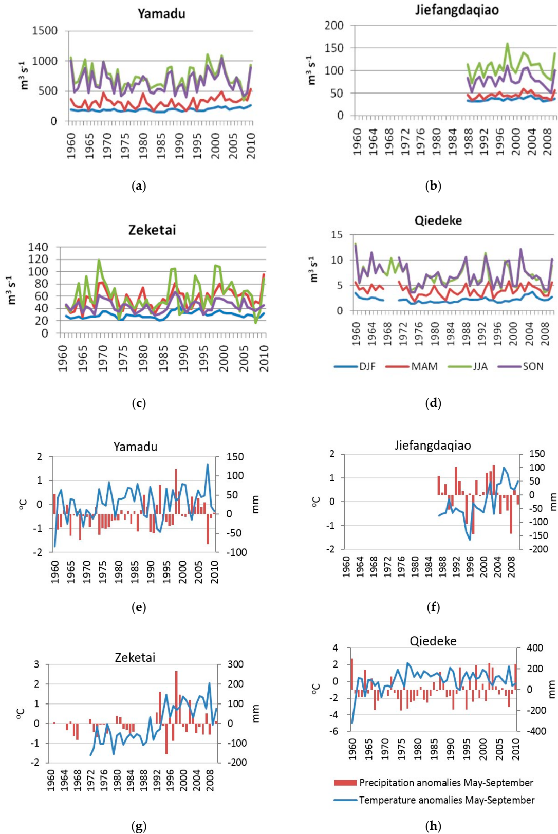
Figure 9. Time series of seasonal mean streamflow ( m^3 s^{-1} ) (a–d) and precipitation and temperature anomalies during the warm season (May to September) (e–h). Note that different scales are used for different rivers.
