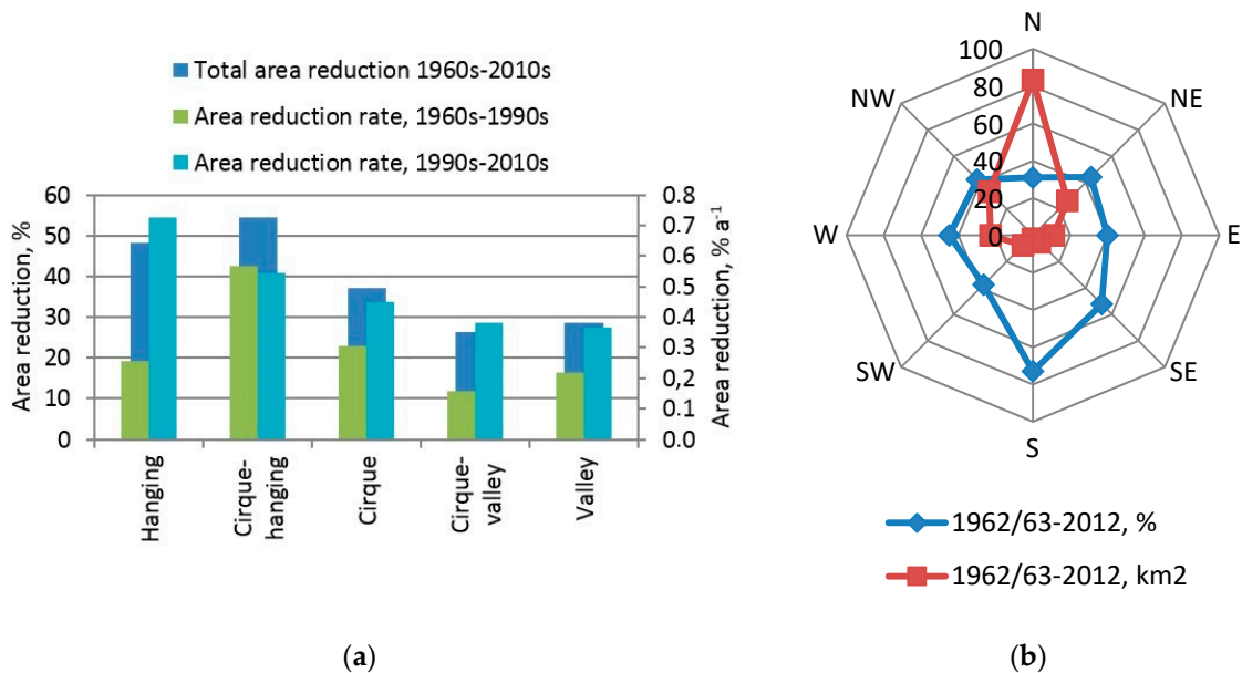
Figure 6. Glacier area loss (a) by morphological types as percentage of the initial glacier area and per year for the two assessment periods, and (b) by aspect.
