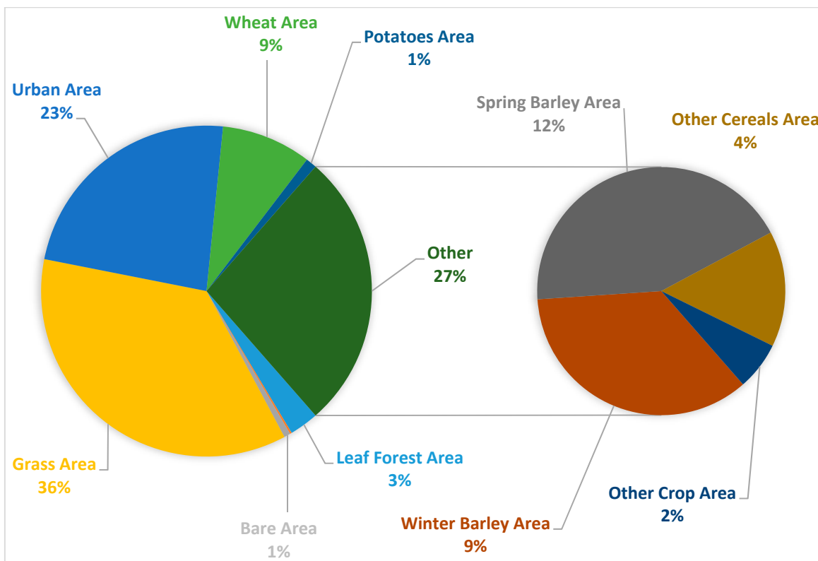
Figure 3. Detailed land use in the Frome catchment.
