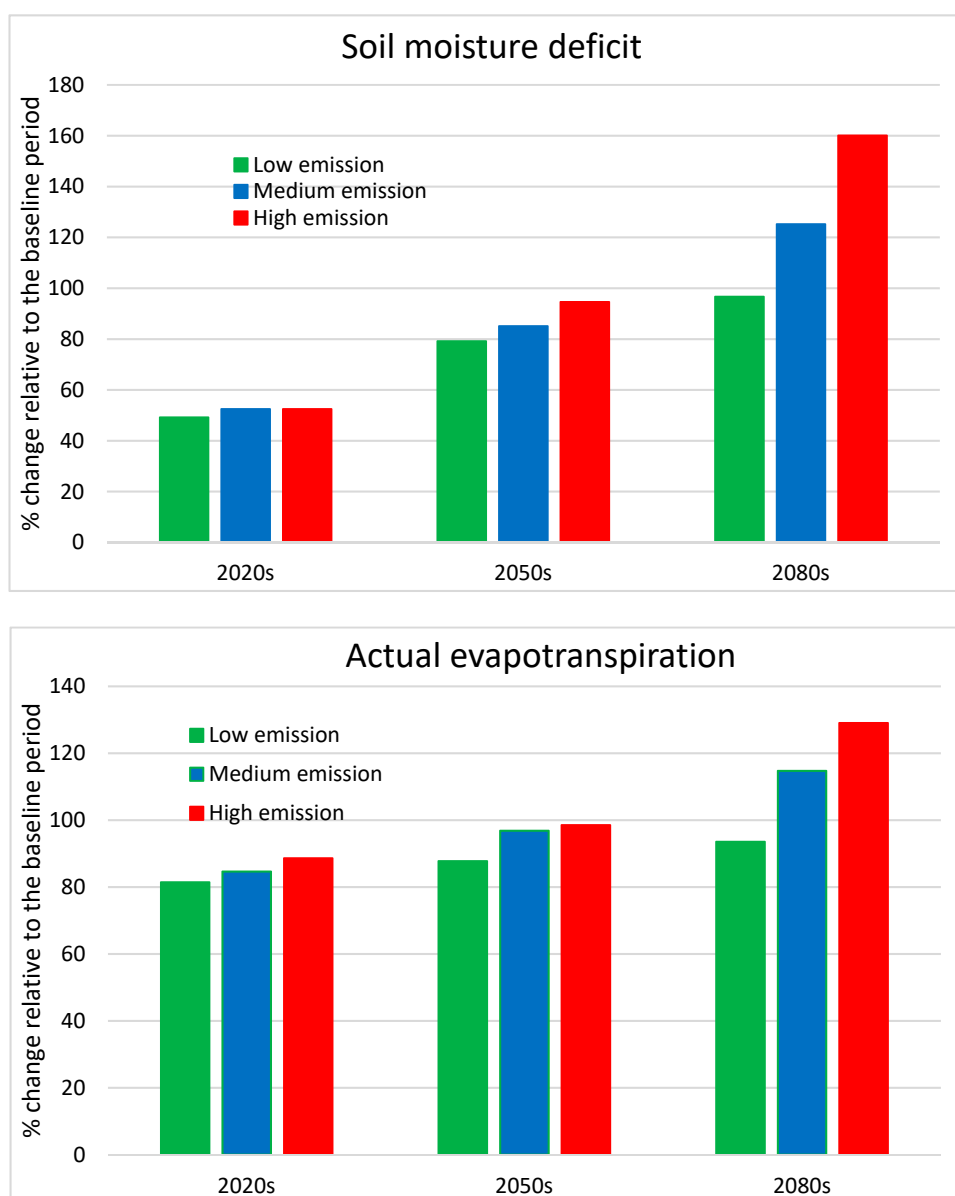
Figure 13. Soil moisture deficit ( top ) and actual evapotranspiration ( bottom ) projected under different climate change scenarios using UKCP09 weather generator data.
