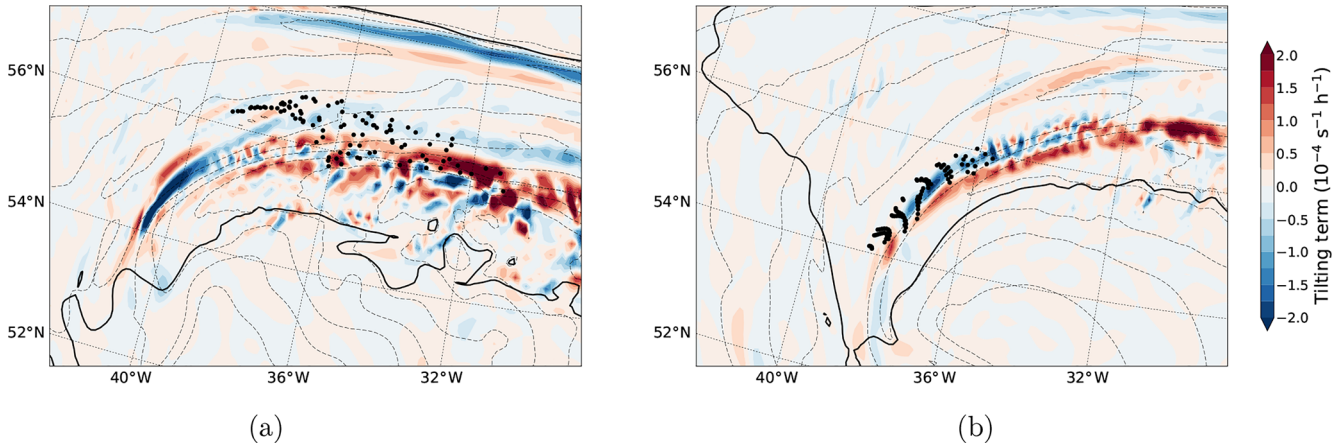
Figure 9. Tilting term of the vertical component of the vorticity equation (shading), \theta_w (thin dashed contours every 1 K) and cloudy regions ( RH_{ice} = 80\% ; black solid contours) at (a) 745 hPa at 81 h from run start and (b) 685 hPa at 86 h. Black dots show the locations of the trajectories. The domain plotted is indicated in Fig. 6b.
