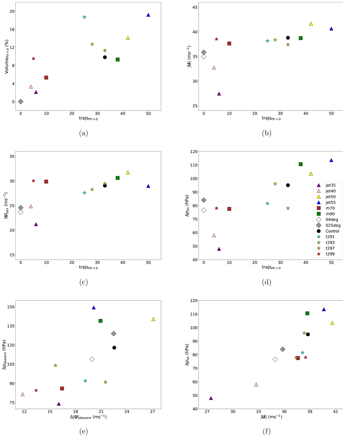
Figure 12. Scatterplots showing, for all the sensitivity experiments, (a) \text{volume}_{PV<0} against \text{traj}_{SPV<0} , (b) |U| against \text{traj}_{SPV<0} , (c) |U|_{\text{sys}} against \text{traj}_{SPV<0} , (d) \Delta p_{5h} against \text{traj}_{SPV<0} , (e) \Delta p_{\text{descent}} against \Delta|U|_{\text{descent}} and (f) \Delta p_{5h} against |U| . \text{traj}_{SPV<0} is the maximum number of trajectories of the 100 selected with negative PV at any instant within 15 h from the time when the trajectories are selected (i.e. identification time), and \text{volume}_{PV<0} indicates the maximum percentage of grid points with negative PV, evaluated in the same time window as \text{traj}_{SPV<0} , in a volume centred on the location of the median of trajectories and extending for 20 grid points in latitude, 40 grid points in longitude and three vertical pressure levels (note that the symbols for the reduced resolution simulations overlie at point (0,0) in panel a). |U| is the maximum Earth-relative speed, |U|_{\text{sys}} is the system-relative speed at the time when |U| is reached, and \Delta p_{5h} is the maximum 5 h pressure increase in a period ending by identification time. \Delta p_{\text{descent}} and \Delta|U|_{\text{descent}} indicate, respectively, total pressure increase and speed increment during the whole SJ descent, whose end is taken at identification time and whose start has to be not more than 12 h before. All these kinematic quantities refer to the median of trajectories.
