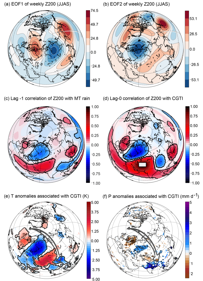
Figure 2. Mid-latitude variability associated with the ISM. (a, b) EOF1 and EOF2 expressed as covariance for the JJAS weekly Z200 field in the Northern Hemisphere ( 0\text{--}90^\circ\text{ N} , 0\text{--}360^\circ\text{ E} ) for the period 1979–2017. (c) Correlation between weekly MT rainfall (lag = 0) and Z200 (lag = -1 week). (d) The CGTI region (white box) and the correlation between CGTI and Z200 (both at lag = 0), which forms the circumglobal teleconnection pattern. In panels (c) and (d), correlation coefficients with a p value of p < 0.05 (accounting for the effect of serial correlations) are shown by black contours. (e) Composite temperature difference between weeks with \text{CGTI} > 1 \text{ CGTI}_{\text{SD}} minus weeks with \text{CGTI} < -1 \text{ CGTI}_{\text{SD}} over the Northern Hemisphere. Panel (f) is as panel (e) but for rainfall anomalies from the CPC-NCEP dataset (as rainfall data for the Pai et al., 2015, dataset are available over India only) for the period 1979–2017. In panels (e) and (f), anomalies with a p value of p < 0.05 (accounting for the effect of serial correlations) are shown by black contours, while grid points which are found significant only with non-corrected p values are shaded.
