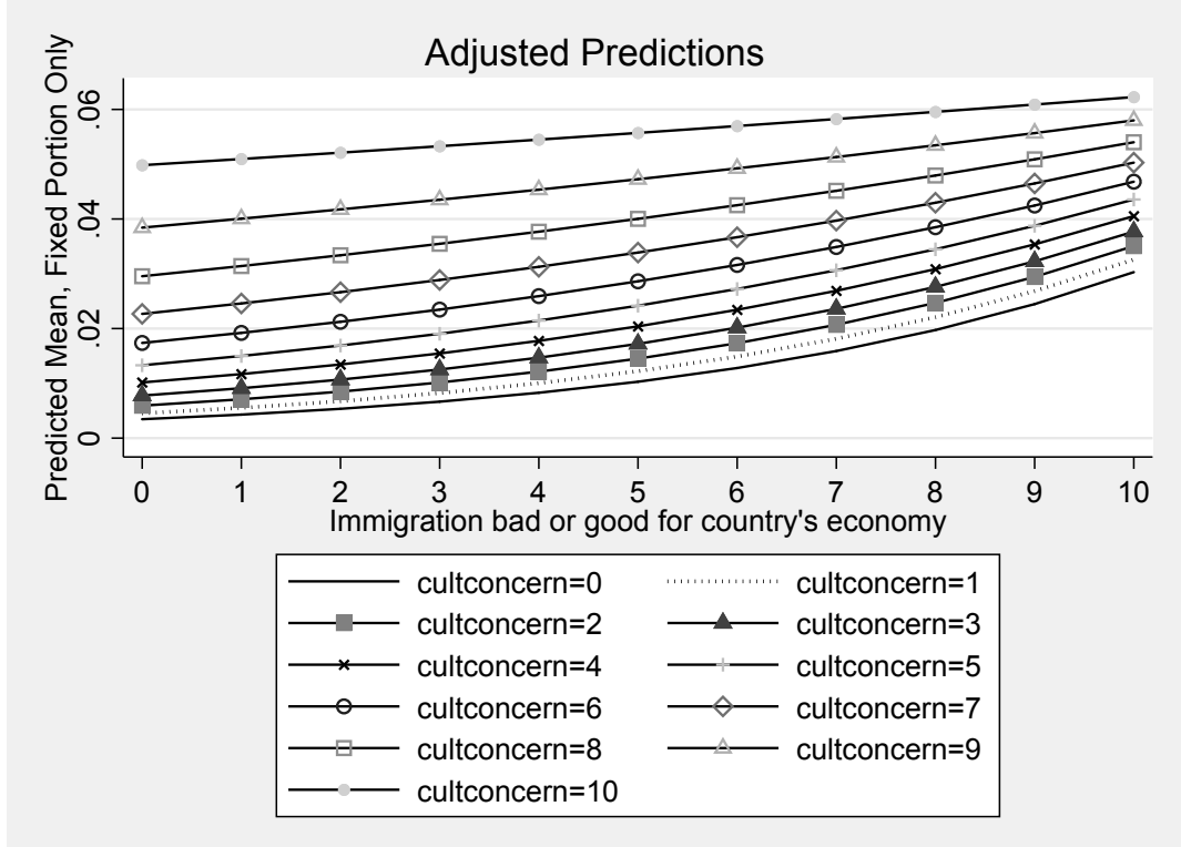
Figure A3.2. Predicted probabilities using column 9 of table A3.1.a
