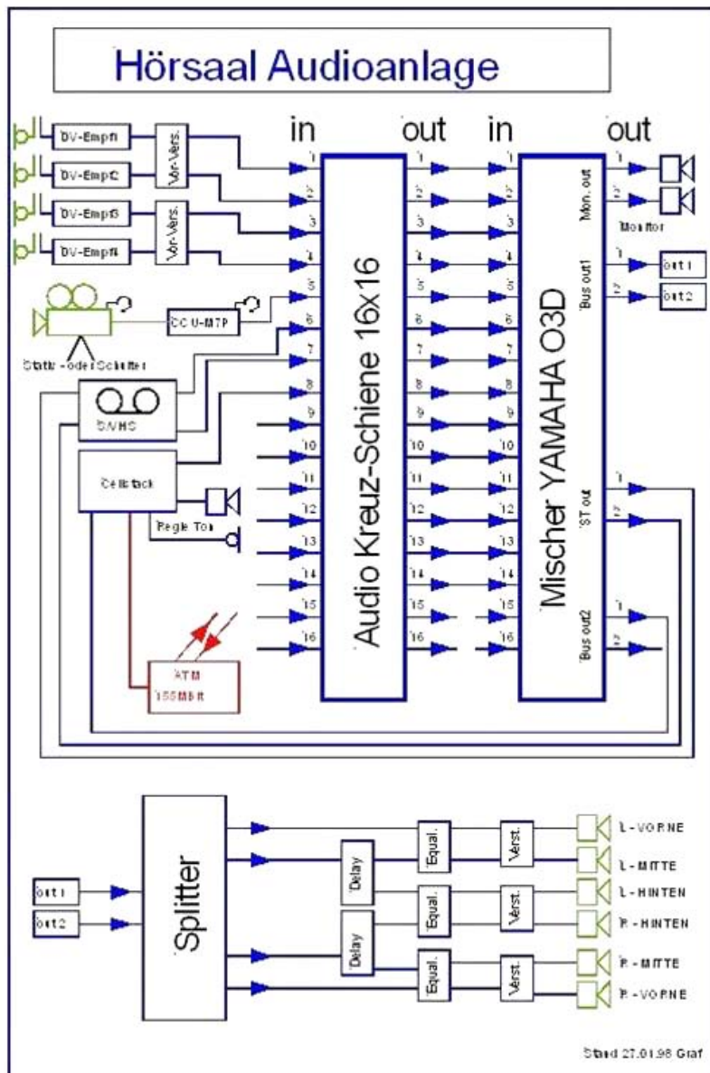
Audio-Konfiguration
