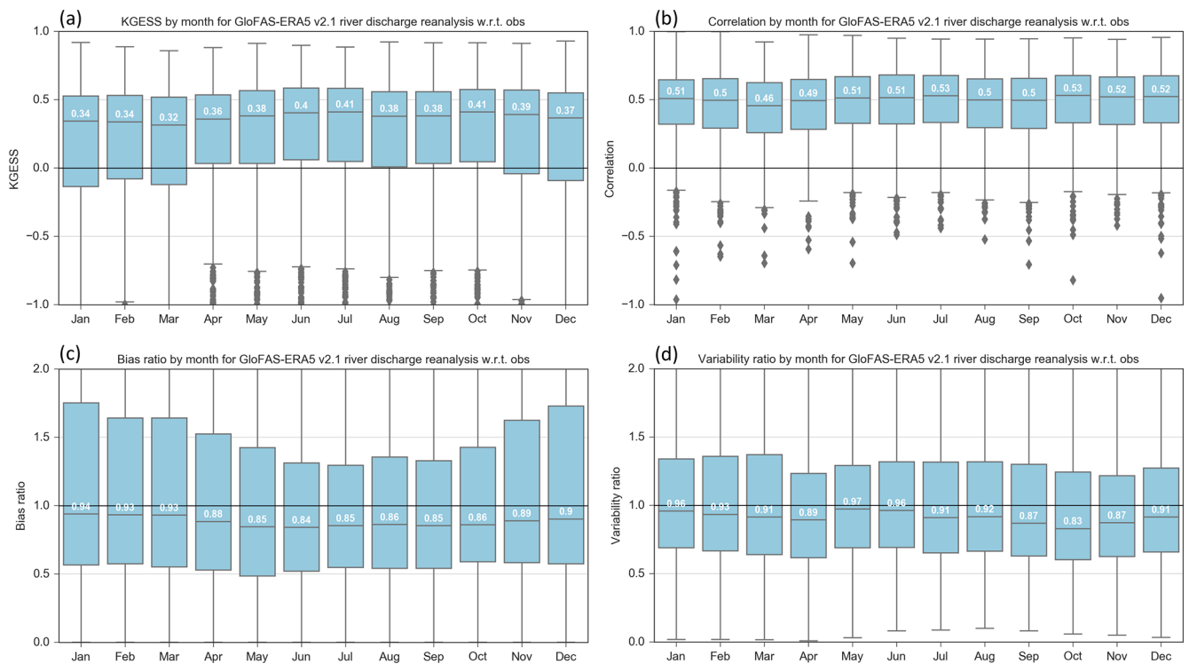
Figure 8. Performance metrics for each month for all 1801 stations. Modified Kling–Gupta efficiency skill score (KGE S ) (a) with decomposition of KGE S into Pearson correlation (b), bias ratio (c), and variability ratio (d). Boxes represent the IQR and horizontal grey line the median. Whiskers extend to the most extreme data point unless the data point is more than 1.5 times the IQR from the box and is instead represented as an outlier (grey diamond).
