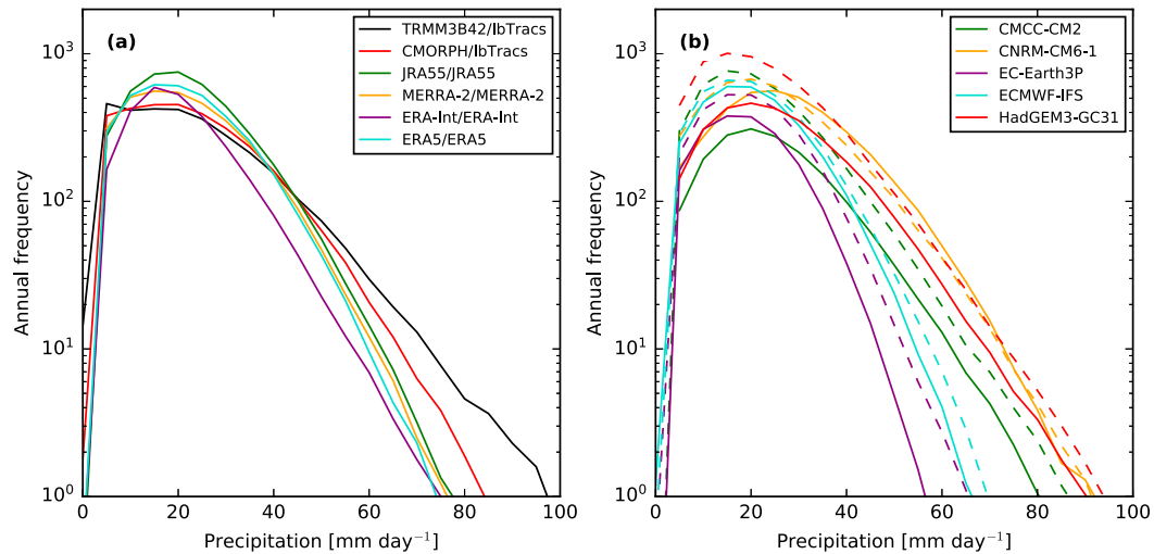
FIG. 2. Mean annual frequency of TCP_{5^\circ} in bins of 5 \text{ mm day}^{-1} in (a) observations and (b) models. In (a) the legend indicates the pair of products used for precipitation and tropical cyclones tracks. Each 6-hourly observation counts for one occurrence. The entire time period available for each model and observation was used to compute the annual mean distribution. Solid lines stand for LR and dashed lines stand for HR.
