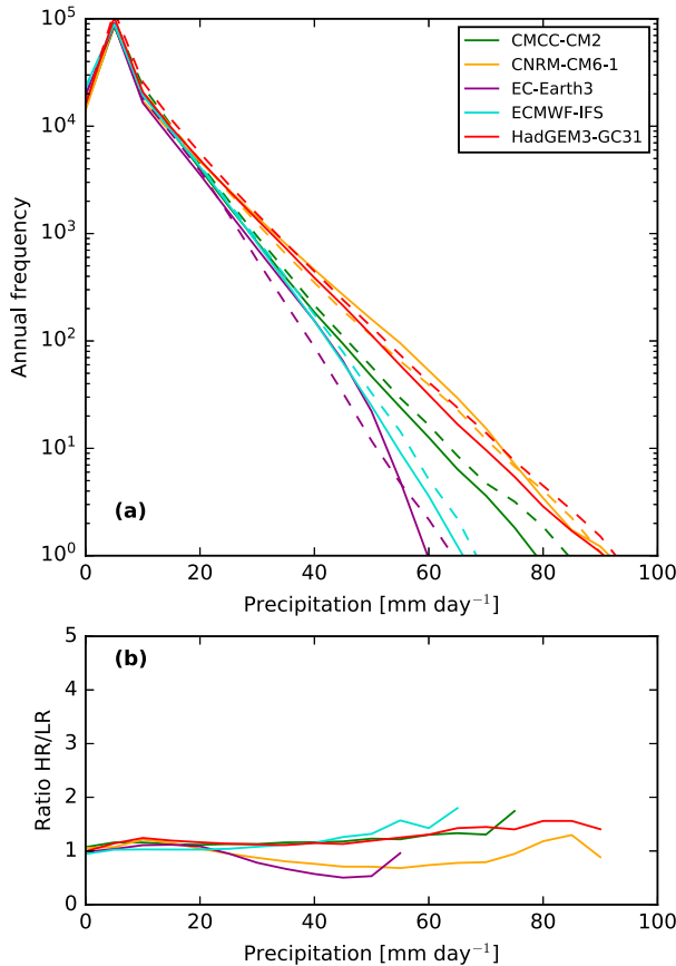
FIG. 3. (a) As in Fig. 2b, but for precipitation associated with all tropical vortices within a radius of 5° from MSLP and (b) the ratio of the distribution between HR and LR.
