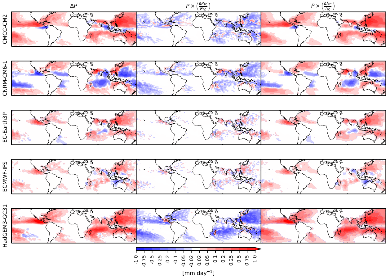
FIG. 6. (left) Difference of precipitation associated with tropical cyclones ( \text{mm day}^{-1} ; occurring in a 5^\circ cap) between HR and LR. Precipitation associated with tropical cyclones (occurring in a 5^\circ cap). The difference of precipitation between HR and LR has been decomposed into two contributions resulting from (center) the change in the amount of precipitation per tropical cyclone and (right) the change of the number of tropical cyclones.
