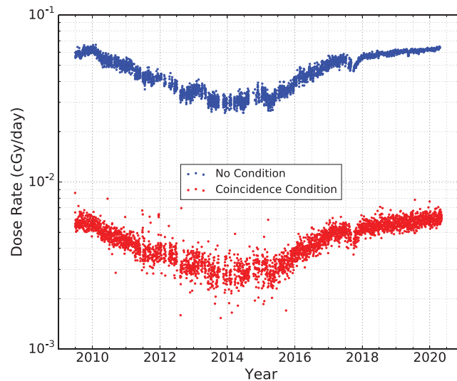
Figure 1. Comparing dose rates measured by D5 and D6 detector pair, projected to free space and converted to show dose rates deposited in water, with and without coincidence conditions. Blue circles represent CRaTER D5 and D6 detector pair dose rates with no coincidence conditions. Red circles represent D5 and D6 detector pair dose rates using the triple coincidence and the deposited energy in D6 > D4 > D2 conditions. These dose rates are also projected to free space to eliminate the effect of the triple coincidence condition limiting the field of view.
