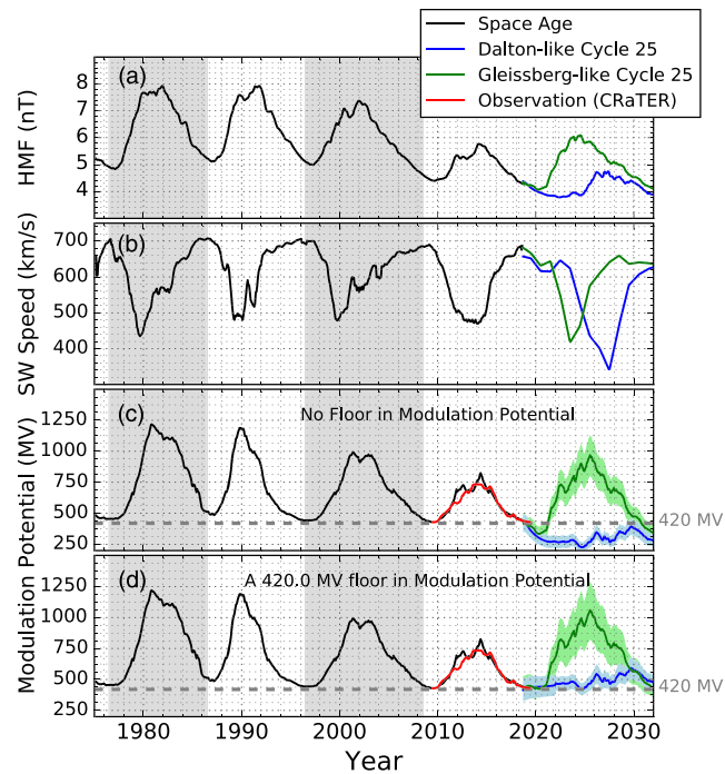
Figure 5. Panel (a) shows the HMF intensity through the space age (black) and extending to a speculated Cycle 25 (blue and green for Dalton-like and Gleissberg-like cases respectively). Panel (b) shows the global solar wind speed from Owens et al. (2017) using the same color code. Panels (c) and (d) show the modulation potential from BON14 through space age (black) and the modulation potential from CRaTER measurements in Cycle 24 (red). The modulation potential for a Dalton-like and a Gleissberg-like Cycle 25 based on the correlation from this work (Figure 4a) is shown in panel (c). Panel (d) shows the modulation potential for these two cases applying the floor in modulation potential from BON14 (using correlations in Figure 4b).
