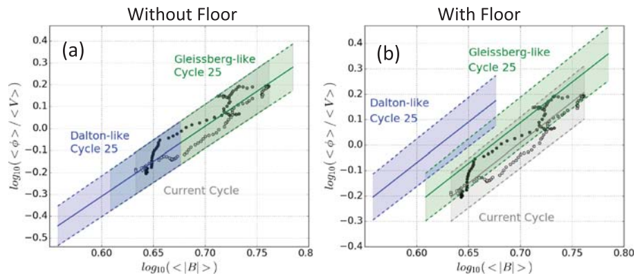
Figure 4. (a) The correlation acquired from Cycle 24 is applied to two possible scenarios for Cycle 25. The HMF strength for a Dalton-like and a Gleissberg-like Cycle 25 is calculated to find the modulation potential for these scenarios using the same slope and intercept from Figure 2. We used blue (green) lines and shaded uncertainty regions to show Dalton (Gleissberg) cases. (b) The same slope from Figure 2 and panel (a) is applied to the speculated Dalton (Gleissberg)-like Solar Cycle 25, applying the floor from BON14 ( \phi = 420.0 MV ).
