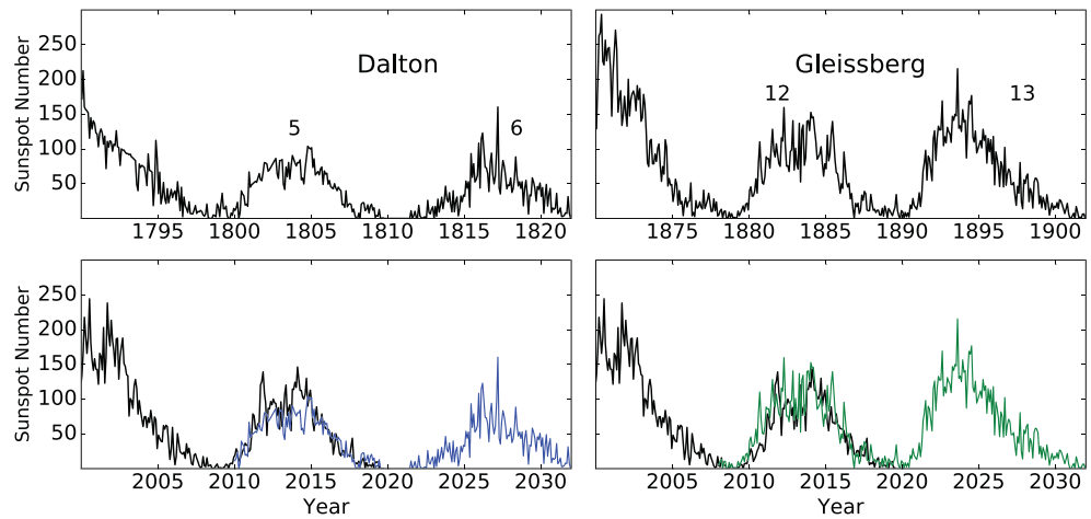
Figure 3. The recent decline in solar activity is compared to previous secular minima. The top left panel shows Cycles 5 and 6 (Dalton period), and in the bottom left these two cycles are laid over the current cycle. The top right panel shows Cycles 12 and 13 (Gleissberg period). In the bottom right, these two cycles are laid over Cycle 24.
