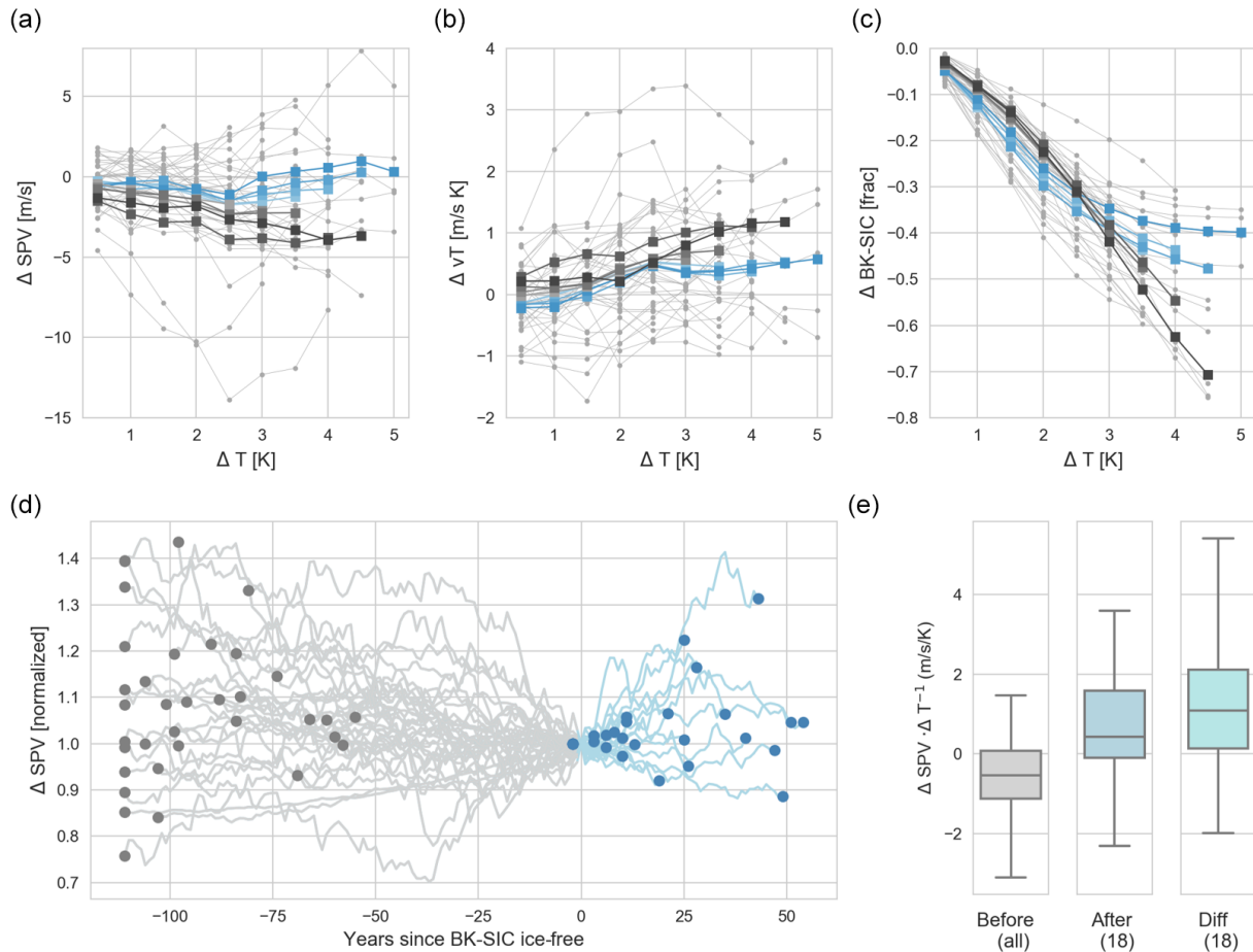
Figure 2. The role of the timing of the BK seas becoming ice-free. (a–c) As in Fig. 1a–c but with the ensemble mean indicated separately for the subsets of models where the BK seas become ice-free early (before 2090, blue lines) and those which are ice-free late (after 2090, dark grey lines). (d) Time series of moving 30-year mean SPV normalized by the 30-year mean reached before the BK seas become ice-free (in OND). Grey lines thus show the evolution of change when there is sea ice and blue lines for when BK is ice-free. Dots indicate the values at the end (blue) and at the start (grey). (e) Boxplot of SPV change before and after BK is ice-free (normalized by global mean warming level over the respective period), as well as the difference for each model. The boxes indicate the inter-quartile range, and the whiskers represent the upper and lower quartile ranges. Only models which were ice-free for at least 10 years (i.e. before 2090) are included in the latter two boxplots (in total 18 models). In all panels, changes were calculated relative to the 1960–1989 reference period (see also Sect. 3).
