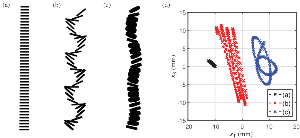
FIGURE 5 Examples of digital reconstructions of the trajectory of thin falling discs in the (a) steady, (b) periodic and (c) chaotic regime with t/D = 0.1, 0.1 and 0.2 , respectively. (d) The trajectory of the COM within the horizontal x_1 - x_3 plane for each of the examples shown (see legend)
