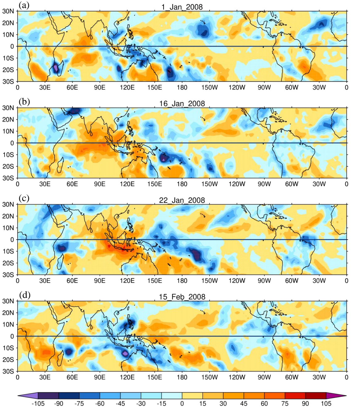
Figure 11 OLR for four days in DJF 2007-08. The OLR is averaged over the specified day and the previous 2 days. The unit for the 3-day OLR average is W m^{-2} .
