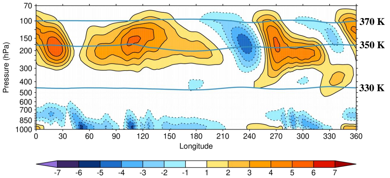
Figure 4 Thirty-year DJF time-mean meridional wind ( \text{m s}^{-1} ) averaged between 5^{\circ}\text{S} and 10^{\circ}\text{N} . Also shown are the isentropic levels 330 K, 350 K and 370 K.
