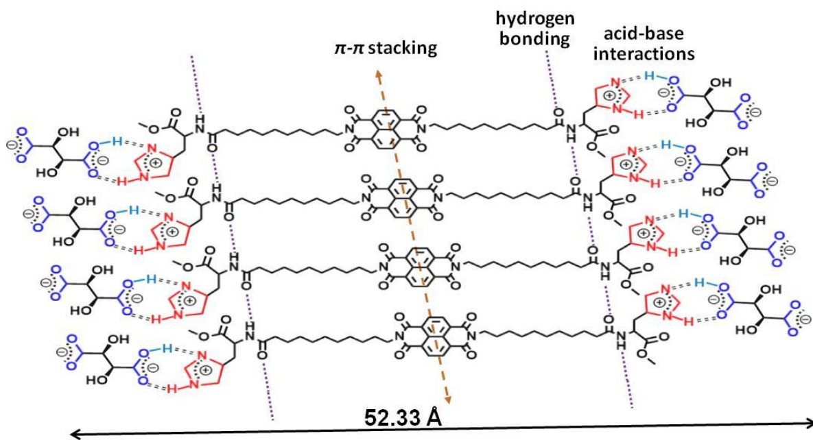
Figure 5: Probable packing model for NDIP and tartaric acid based two component self-assembled system in aqueous medium and \text{---}\text{---}\text{---}\text{---} lines indicate hydrogen bonding.
