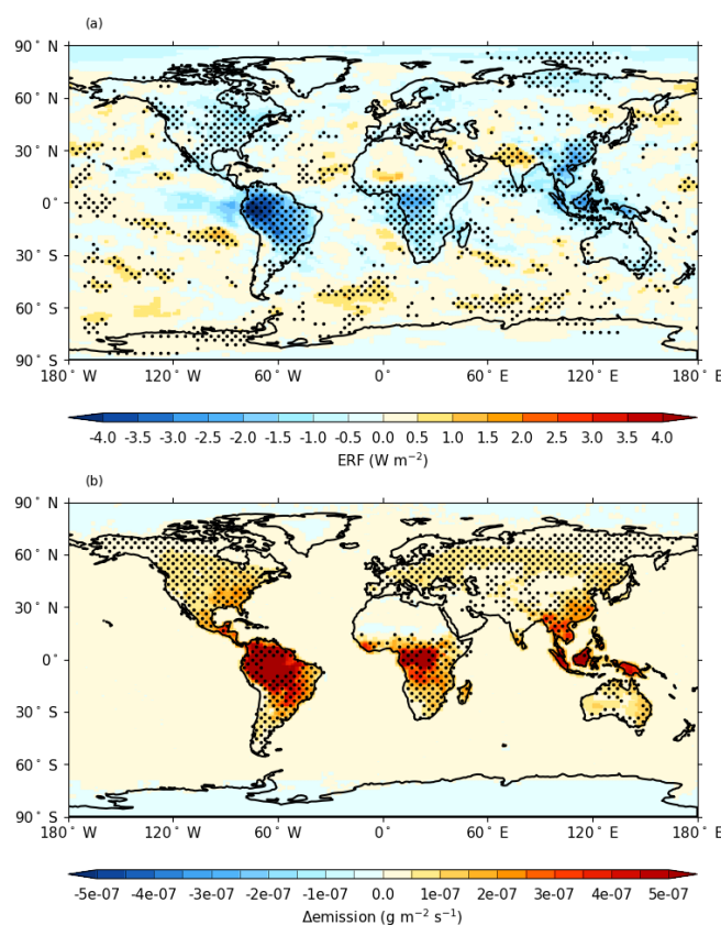
Figure 4. Multi-model mean (a) ERF from pi\text{Clim-}2x\text{VOC} vs. pi\text{Clim-control} , (b) change in BVOC emissions for abrupt-4x\text{CO}_2 vs. pi\text{Control} . Stippling shows areas where the mean changes by more than the standard deviation across models.
