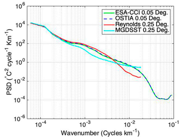
FIG. 2. Power spectral density at the equator in the Pacific Ocean (0°N, 120°E–80°W) for ESA-CCI (green), OSTIA (dashed dark blue), NOAA Daily OISST (Reynolds 0.25°; red), and MGSST (cyan) based on the daily temporal and original spatial resolution for the period 1982–2018.
