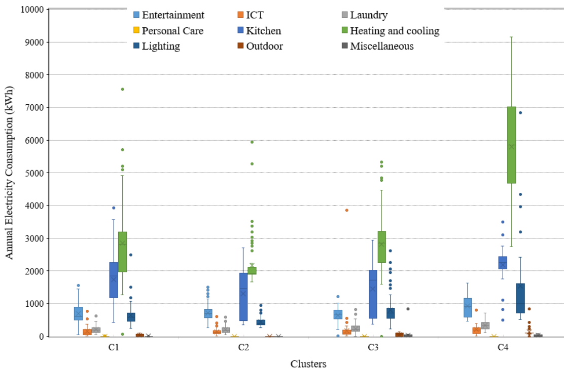
Fig 10: Energy Consumption of Clusters by Appliance Category
