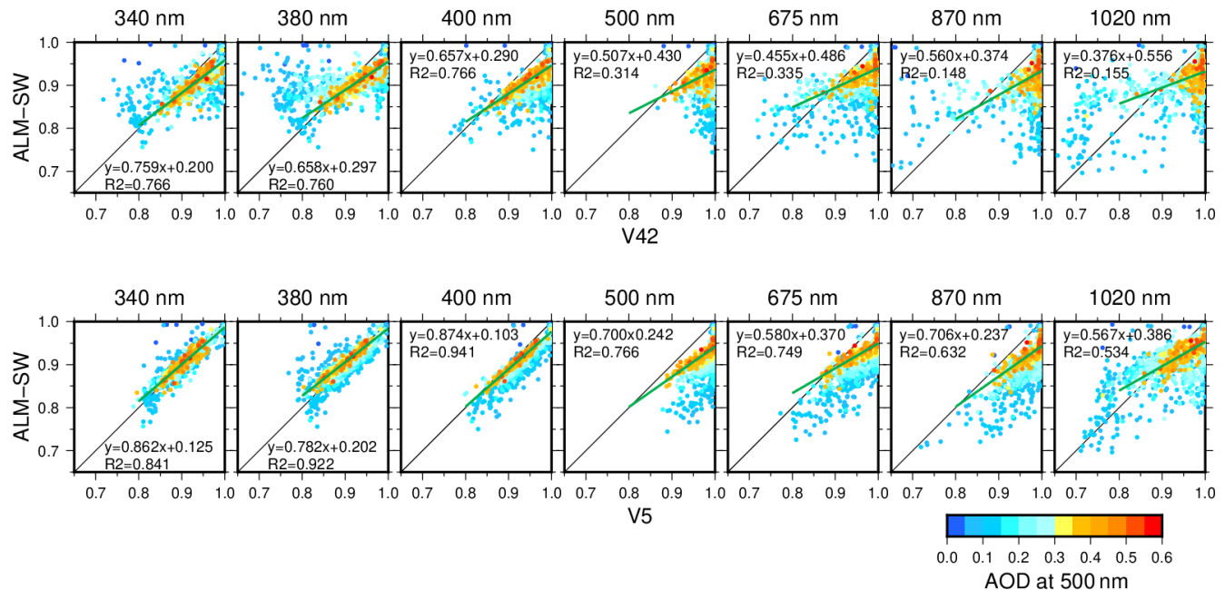
Figure 10. Comparisons of the single-scattering albedo between ALM-SW, V42, and V5. Colors indicate the aerosol optical depth at 500 nm; y = ax + b and R^2 are the linear fitting and the coefficient of determination for the data relating to an aerosol optical depth of more than 0.3.
