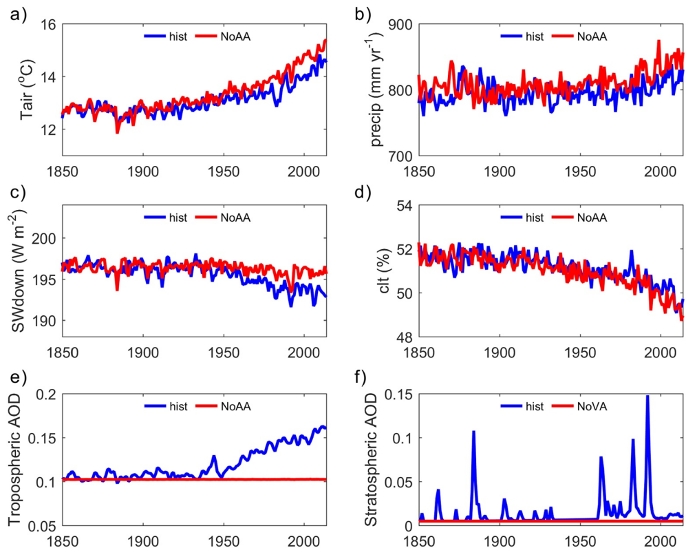
Figure 2. The bias-corrected annual-mean climate temporal evolution over terrestrial regions from the historical (blue lines) and histNoAA (red lines) simulations (a)–(e). The red line in (f) represent a scenario with no volcanic eruptions. (a) Air temperature; (b) Precipitation; (c) Downward shortwave radiation; (d) Total cloud fraction; (e) Tropospheric aerosol optical depth; (f) Stratospheric AOD. AOD, aerosol optical depth.
