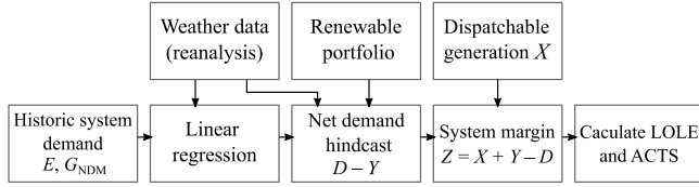
Fig. 1. High-level modelling approach. The net demand D - Y is calculated for a given year by combining a linear model of historic system electrical and Non Daily Metred (NDM) gas demand E, G_{\text{NDM}} with coincident renewable generation Y . This is combined with dispatchable generation X , from which Loss of Load Expectation (LOLE) and Additional Capacity to Secure (ACTS) can be calculated. The NDM gas demand is used as a proxy for space heating demand.
