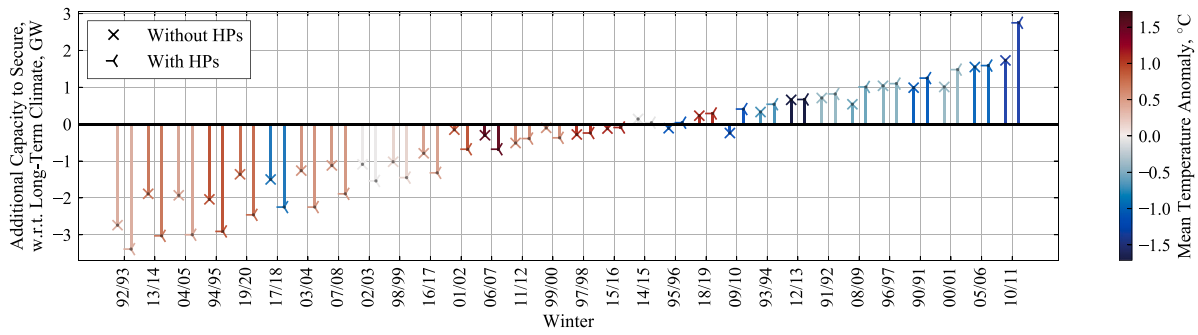
Fig. 8. Changes in ACTS, comparing values if all years have the same weather against the 30-year climate, calculated for the \tau - 4 delivery (24/25). The addition of heat pumps leads to an increased range of ACTS with respect to the long-term winter climate, due to increased weather sensitivity; although, it is clear that the mean temperature anomaly only partially explains the change in ACTS of individual winters.
