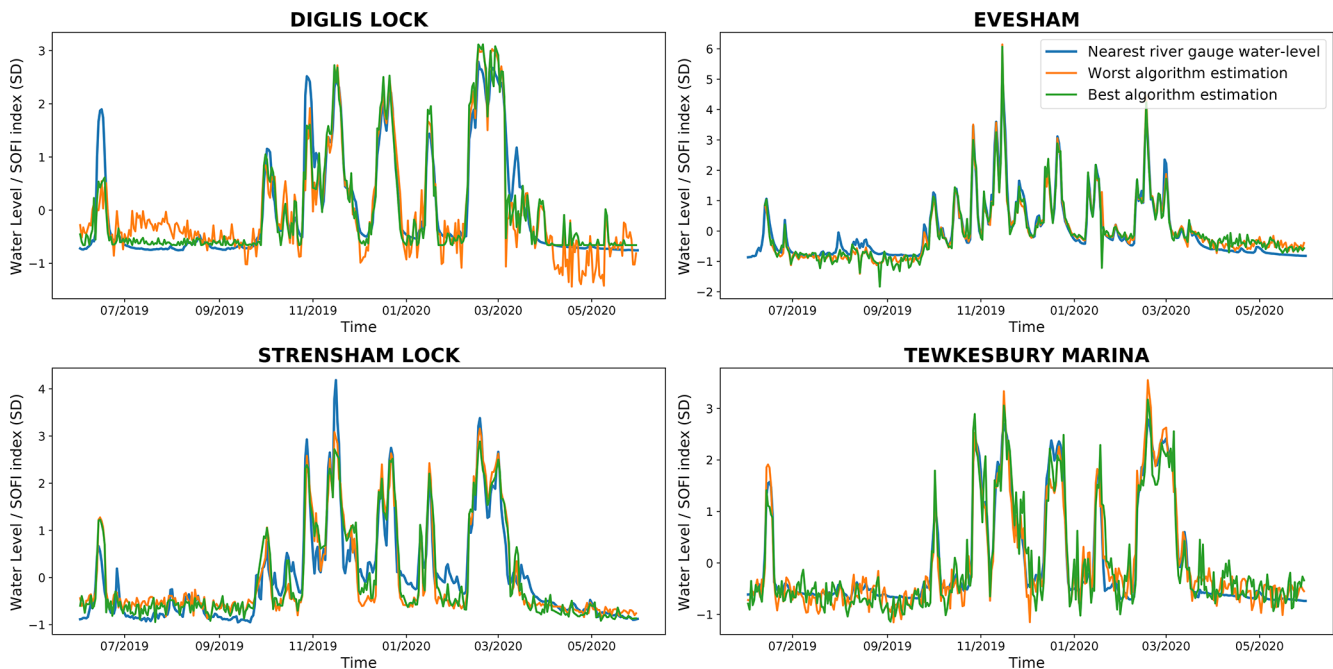
Figure 10. Standardised SOFI of the best window from the 4 × 4 grid in comparison with standardised water levels from nearby river gauges.
