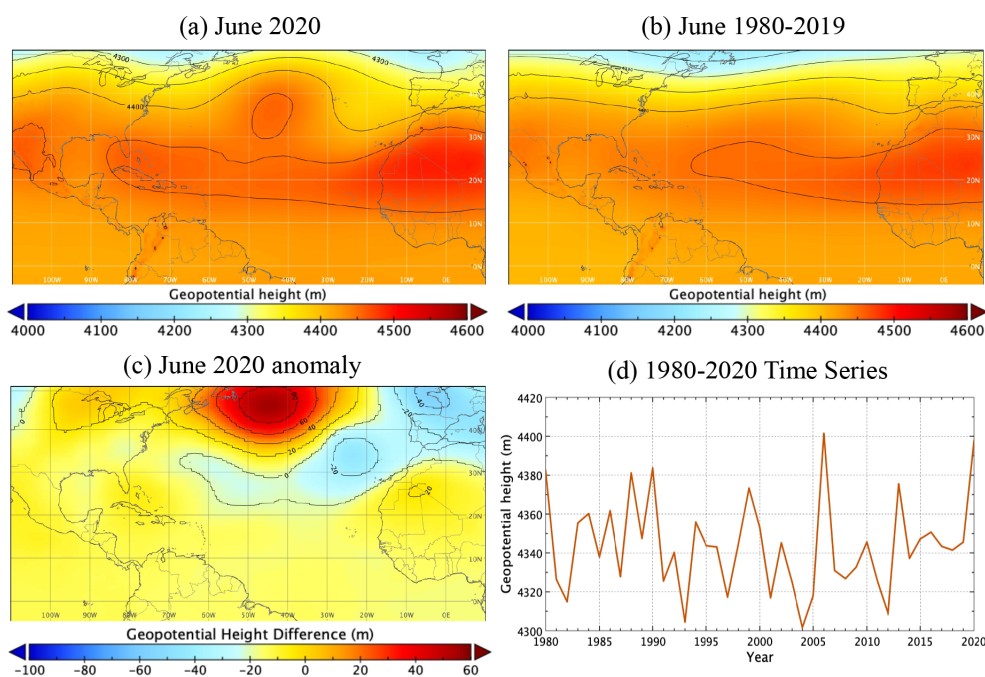
Figure 12. MERRA-2 reanalysis geopotential height at 600 hPa: (a) June 2020, (b) June climatology (1980–2019), (c) June 2020 anomaly, and (d) 1980–2020 time series averaged over 35–50° N and 60–30° W.
