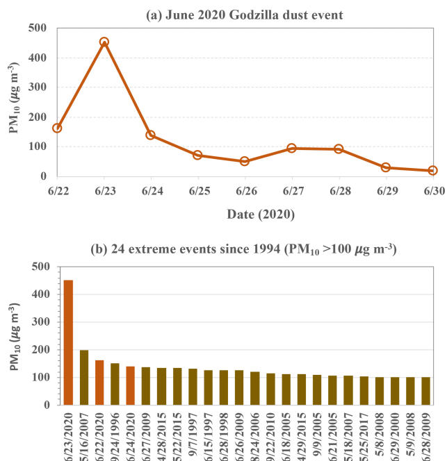
Figure 6. (a) PM 10 concentration measured at Catano, Puerto Rico, during the June 2020 dust event, (b) 24 extreme dust events (PM 10 > 100 µg m -3 ) at this site since 1994.
