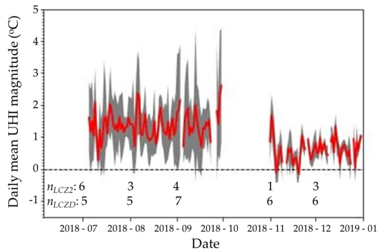
Figure 8. The daily mean urban heat island magnitude (defined as \text{TLCZ2} - \text{TLCZD} ), indicated by the red line. n_{LCZ2} and n_{LCZD} represent the most common number of stations for that month in LCZ 2 and LCZ D, respectively. The filled grey area shows the area between the mean plus one standard deviation and the mean minus one standard deviation.
